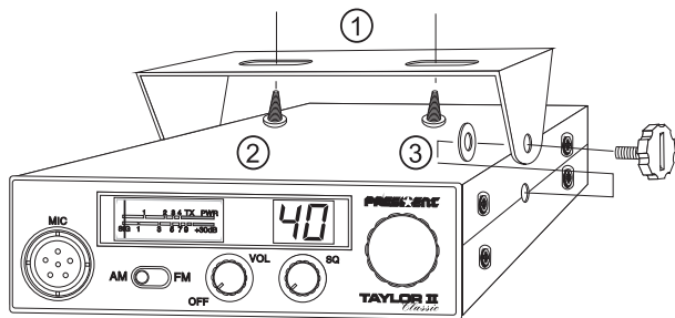
MOUNTING DIAGRAM
